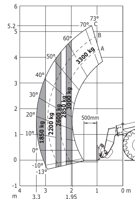
MLA-T 533-145 V+ Following norm EN 474-3 (80%)
